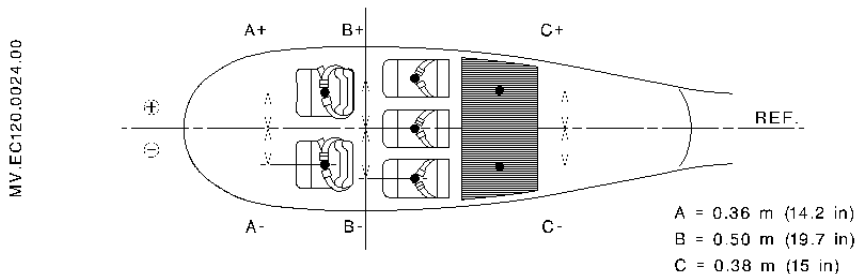
Figure 1: Lateral location of seats and loads
