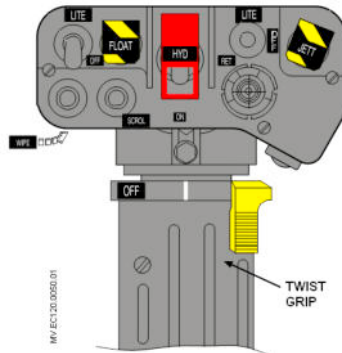
Figure 1: Collective grip
