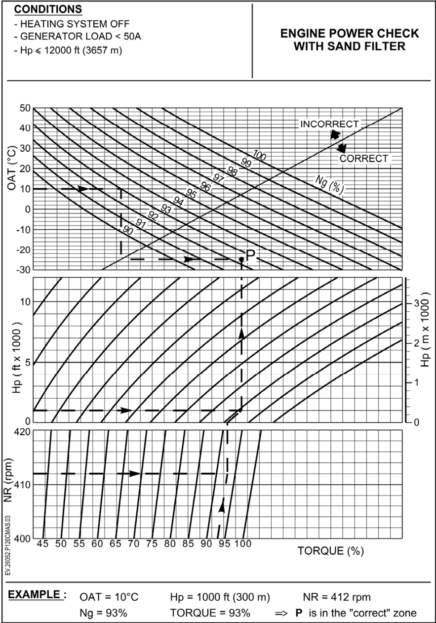
Figure 1: Engine power check with sand filter
