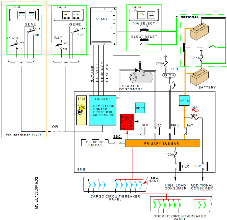
Figure 1: Electrical system
