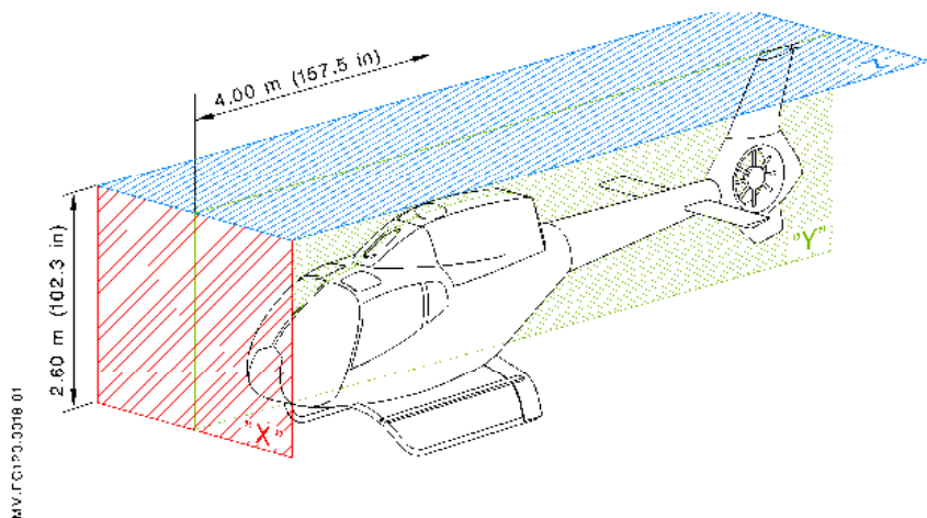
Figure 1: Basic datum planes
