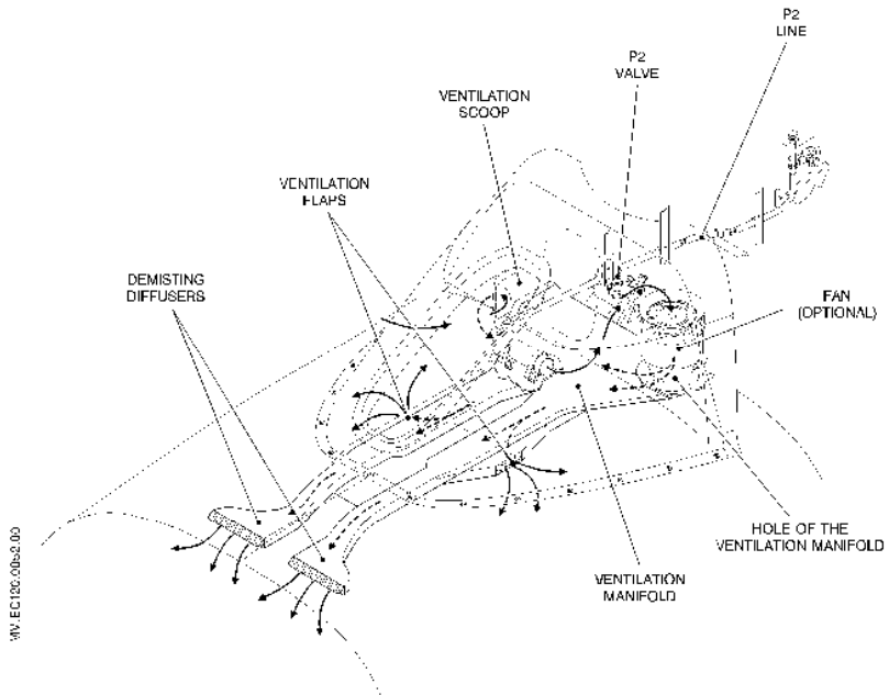
Figure 1: Air generation
