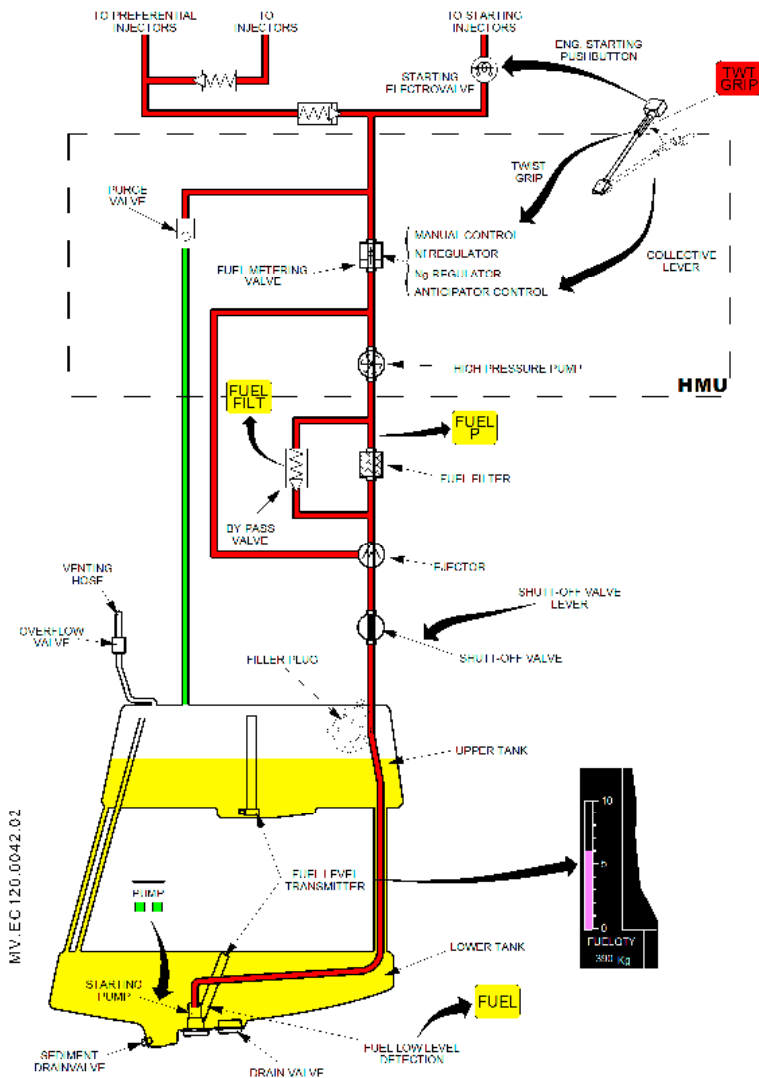
Figure 1: Fuel system
