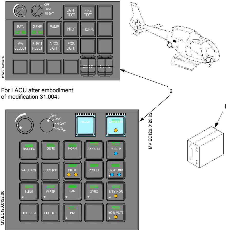
Figure 2: Central computers
