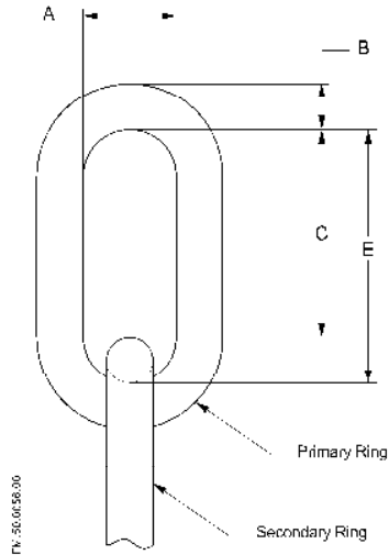
Figure 1: Cargo ring
