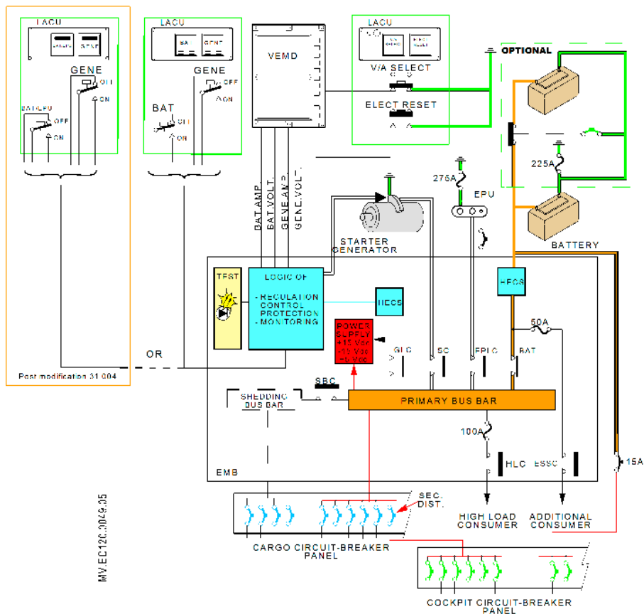
Figure 2: Electrical system
