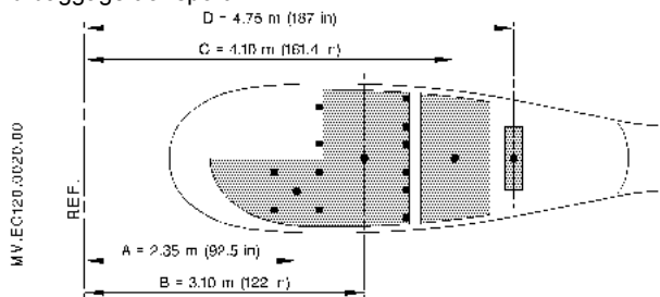
Figure 2: Longitudinal location of loads
