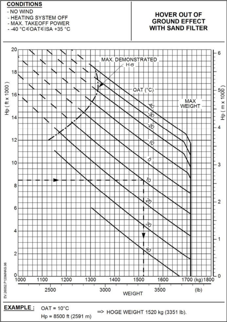
Figure 3: HOGE with sand filter
