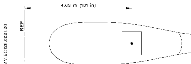
Figure 3: Longitudinal location of fuel
