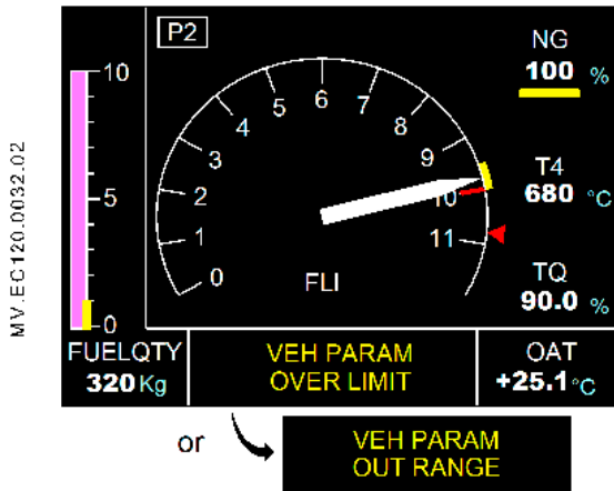
Figure 4: FLI page (Values given as an example) Fuel gauge with auxiliary tank installed (optional)
