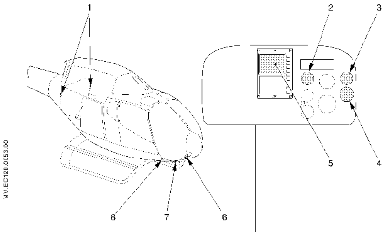
Figure 1: Pitot static system
