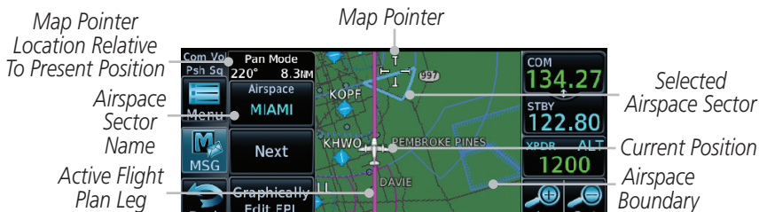
Figure 12-17 Airspace Sectors
