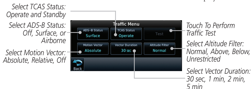
Figure 9-11 ADS-B Traffic Menu
