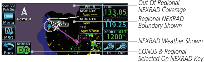
Figure 11-80 Weather Page With Combined NEXRAD Displayed
