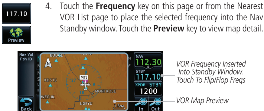
Figure 12-10 Nearest VOR Frequency Entry
