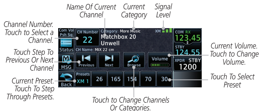
Figure 13-4 Music Menu
