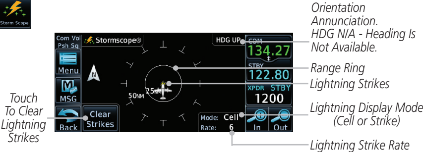
Figure 11-49 StormScope Display (360° Display View Shown)
