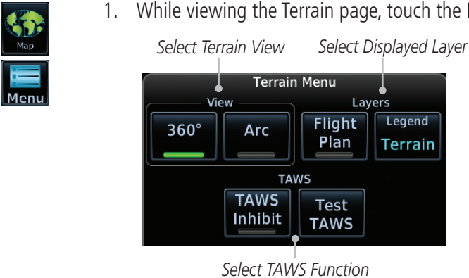
Figure 10-7 Terrain Page TAWS-B Menu
