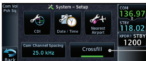
Figure 15-29 Selecting Crossfill
