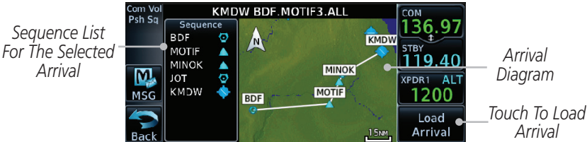
Figure 6-13 Arrival Map Preview and Sequence List
