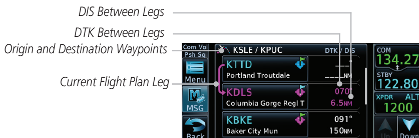
Figure 4-46 Flight Plan Data Fields
