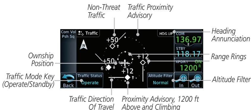
Figure 9-5 Traffic Page
