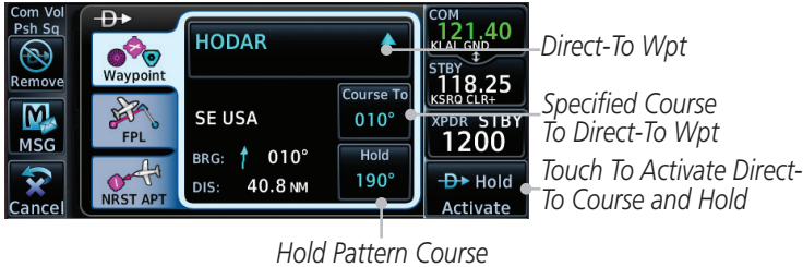
Figure 5-13 Direct-To Page with Hold Selected
