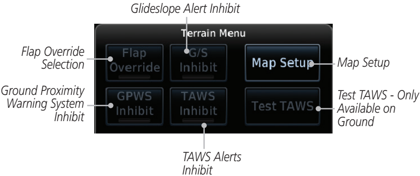
Figure 10-30 TAWS-A Menu
