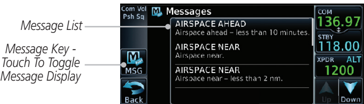
Figure 16-1 Message Display
