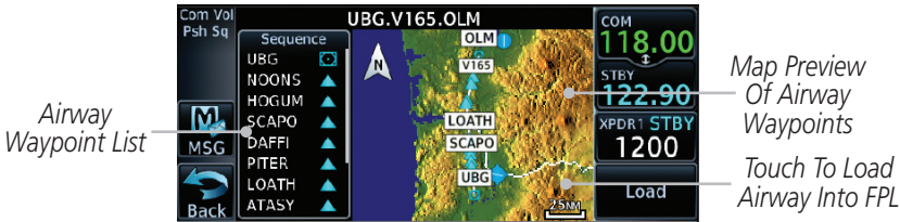
Figure 4-23 Airway Preview
