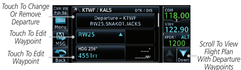
Figure 6-7 Flight Plan View of the Selected Departure
