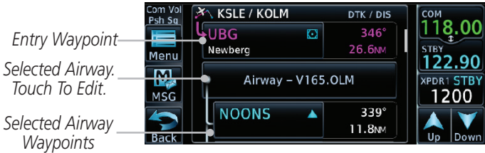
Figure 4-24 Airway Waypoints in the Flight Plan
