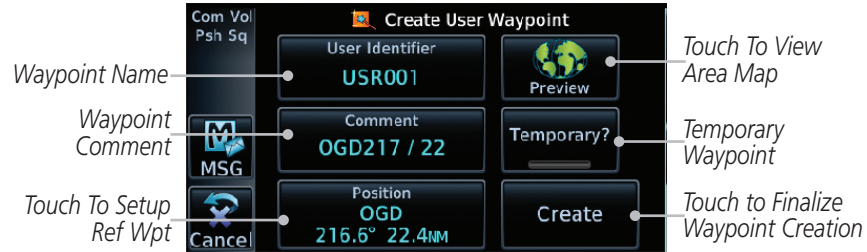
Figure 7-24 Waypoint Info - Create User Waypoint
