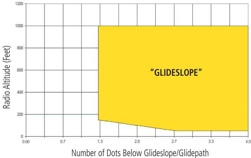
Figure 10-44 Excessive Below Glideslope/Glidepath Deviation Alert Criteria
