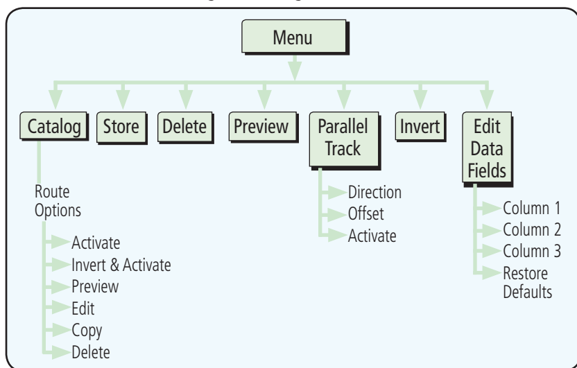
Figure 4-41 Flight Plan Menu Functional Diagram
