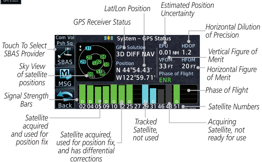
Figure 15-6 GPS Status Page
