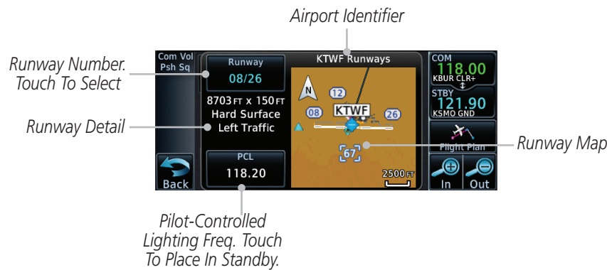
Figure 7-10 Waypoint Info Airport Runway Information Page
