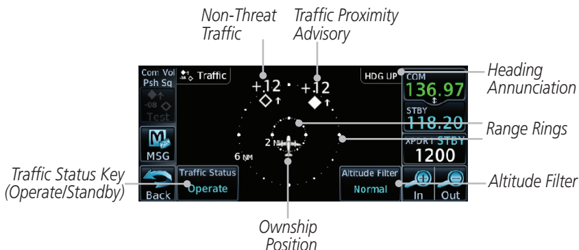
Figure 9-8 Traffic Page
