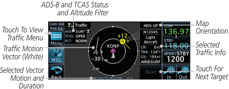
Figure 9-13 Absolute Motion (White Vectors)
