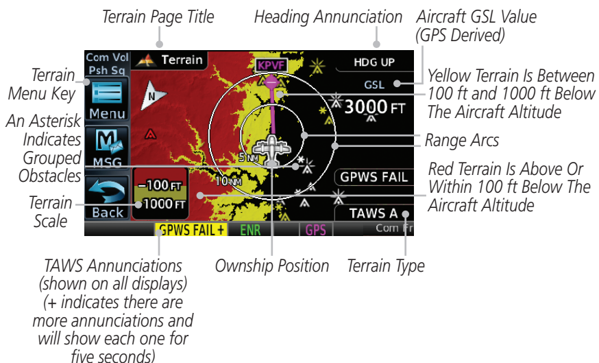
Figure 10-29 TAWS-A Page with 360° View
